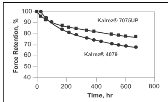
Figure 2. Seal Force Retention at 200°C*
